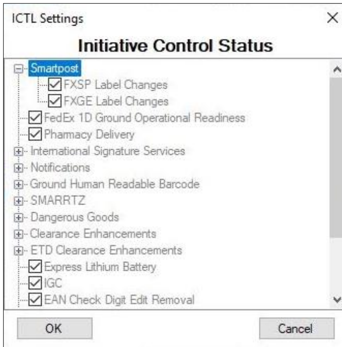
Figure 97: ICTL Settings
