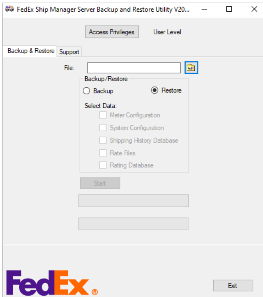
Figure 100: Restore functionality
