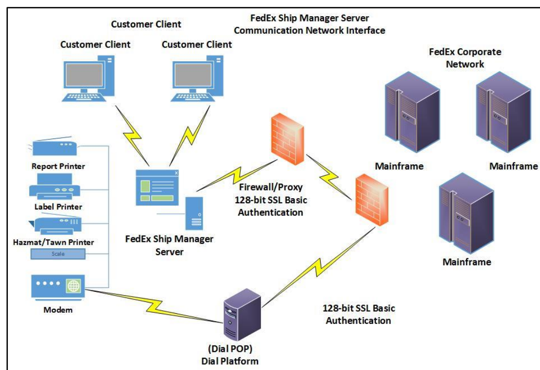
Figure 1: Communication network interface
