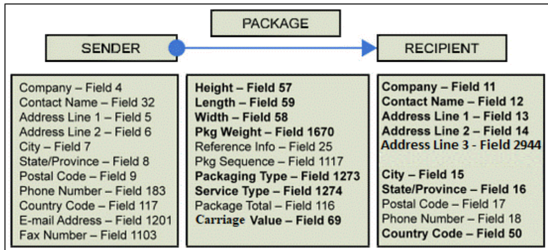
Figure 3: Field information for key elements
