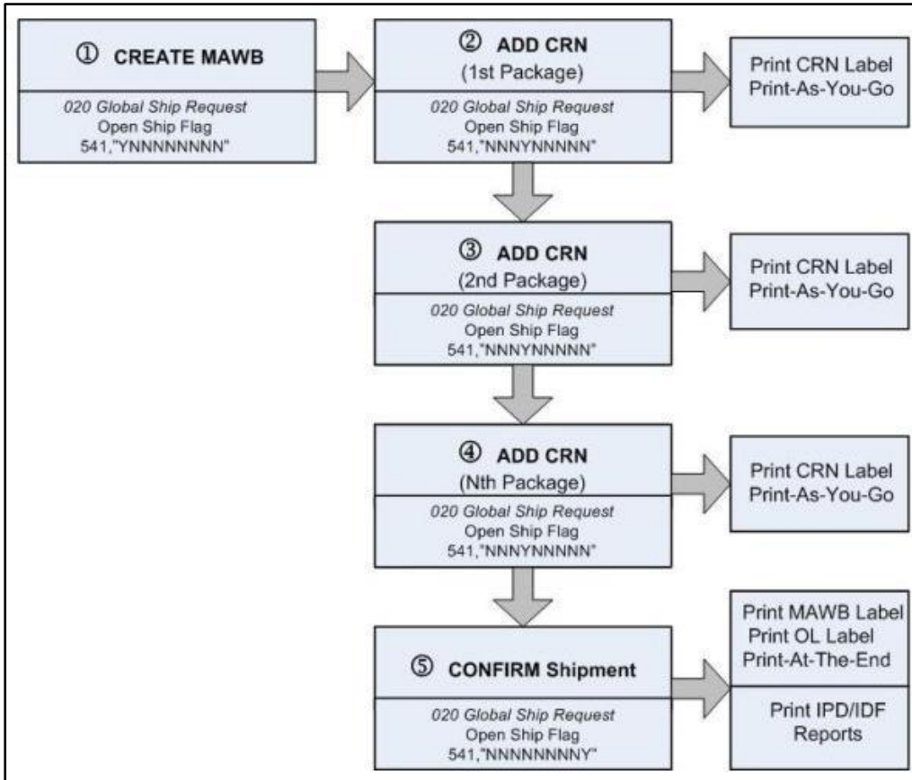
Figure 14: IPD/IDF/IED transaction workflow
