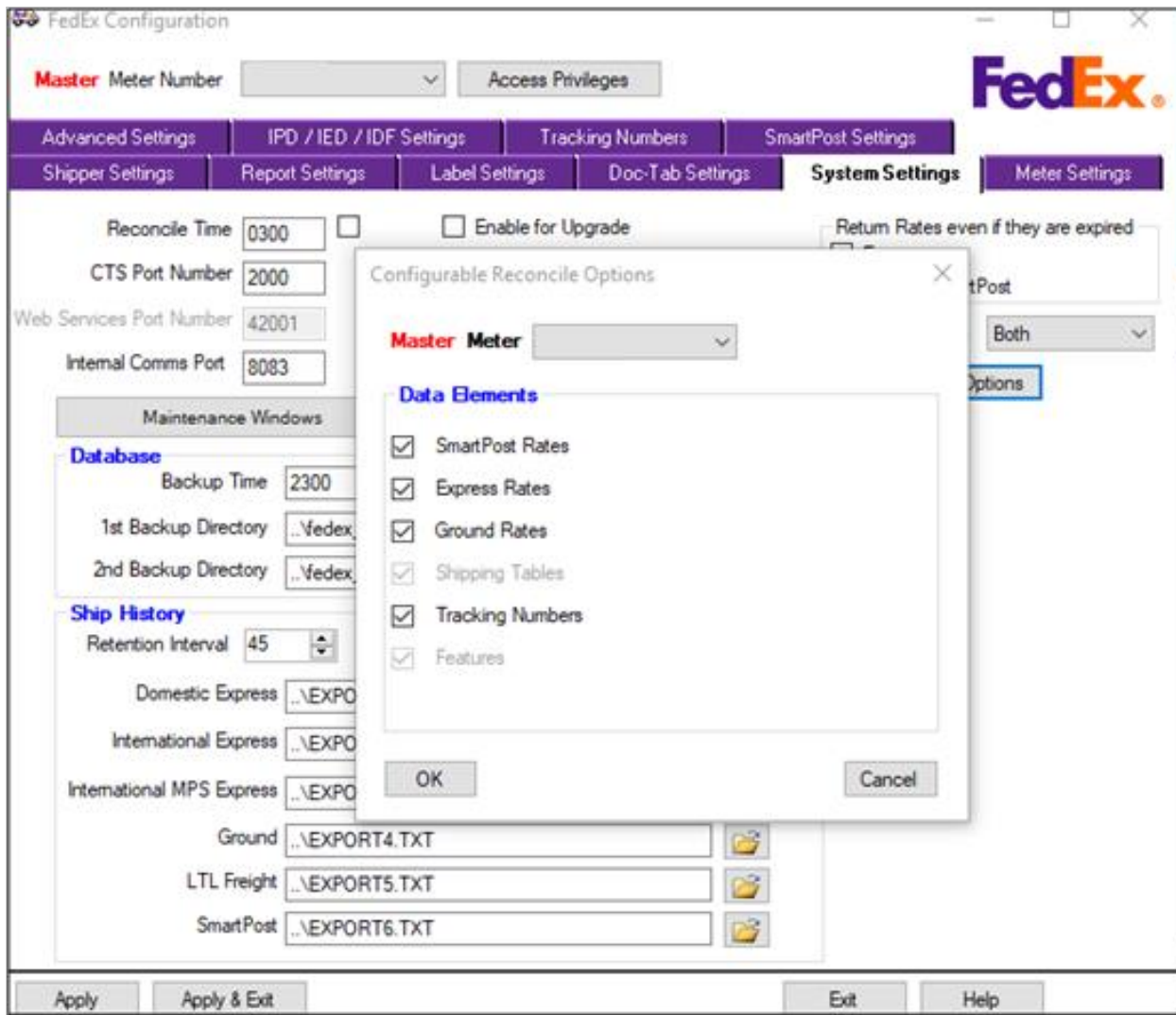
Figure 105: Configure Reconcile options
