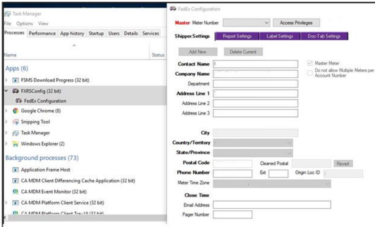
Figure 85: FedEx Ship Manager Config
