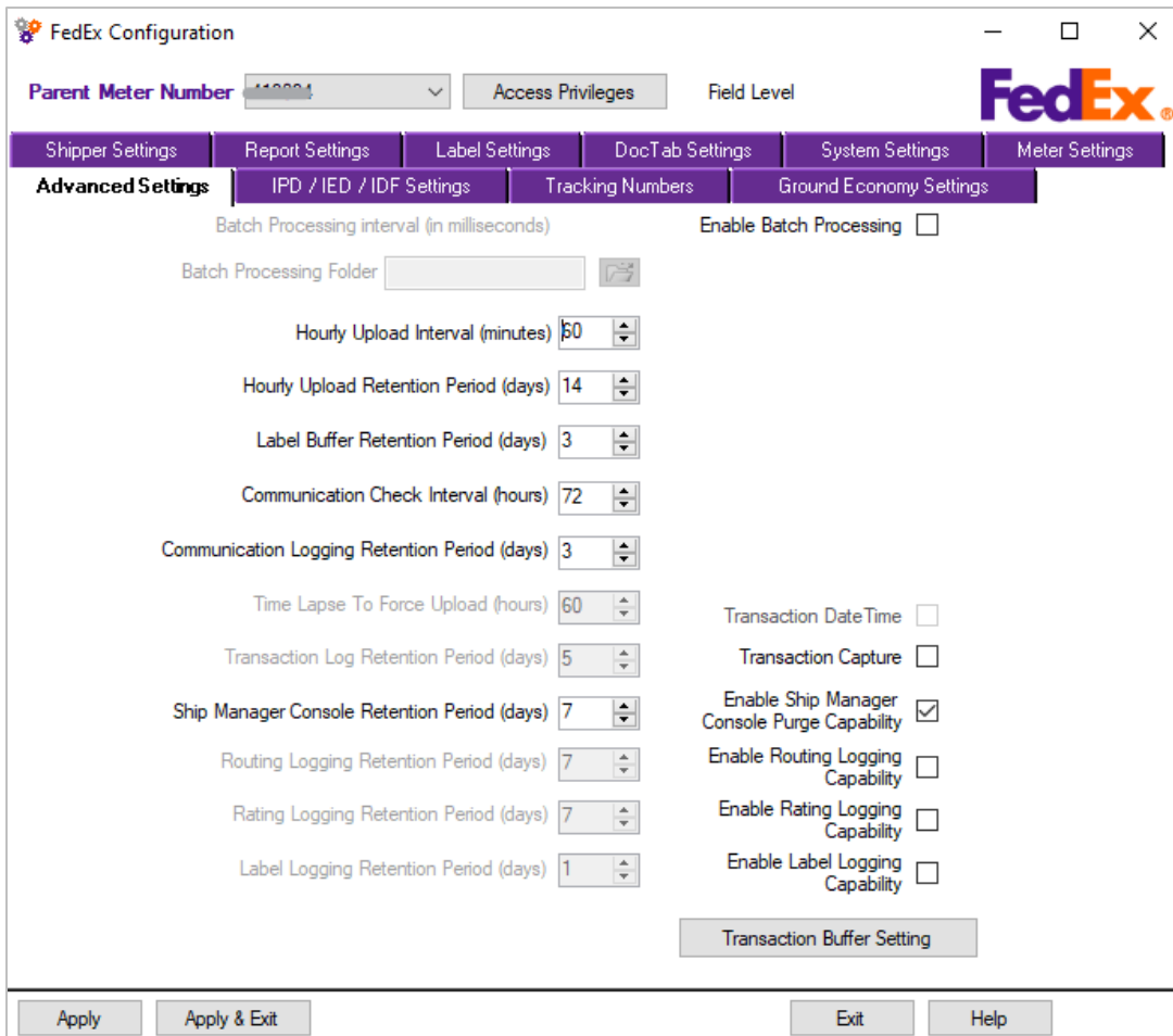
Figure 107: Transaction Buffer Setting in the “Advanced Settings” tab
